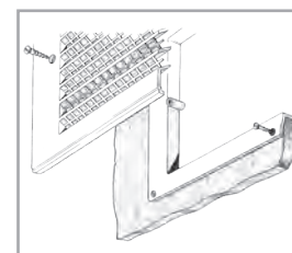
Flushmount Installation
